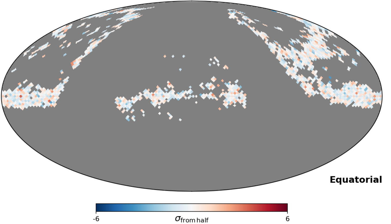
(b) Chirality \sigma_{\text{from half}} per pixel ( n_{\text{spiral}} \geq 200 ; z \leq 0.24 )
