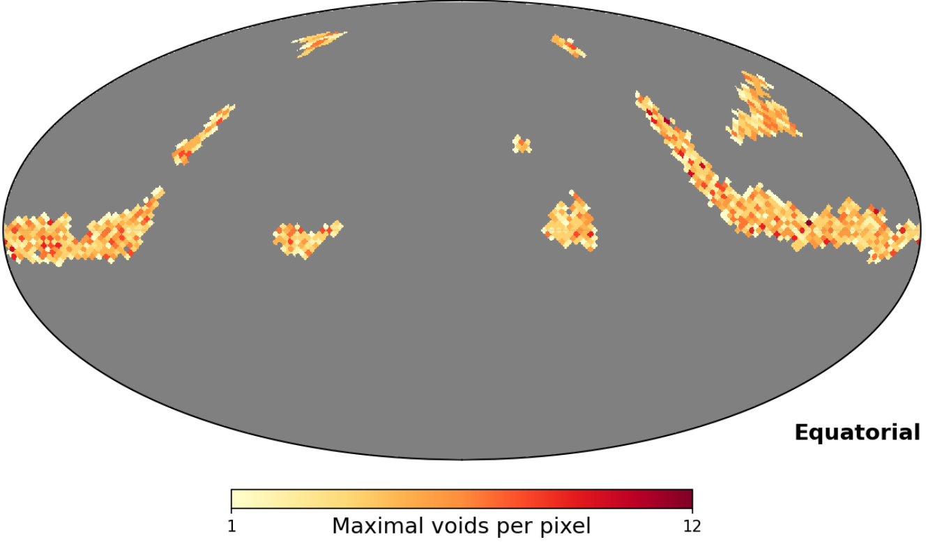
(a) DESIVAST maximal voids per pixel (NSIDE=32; 885 occupied pixels)
