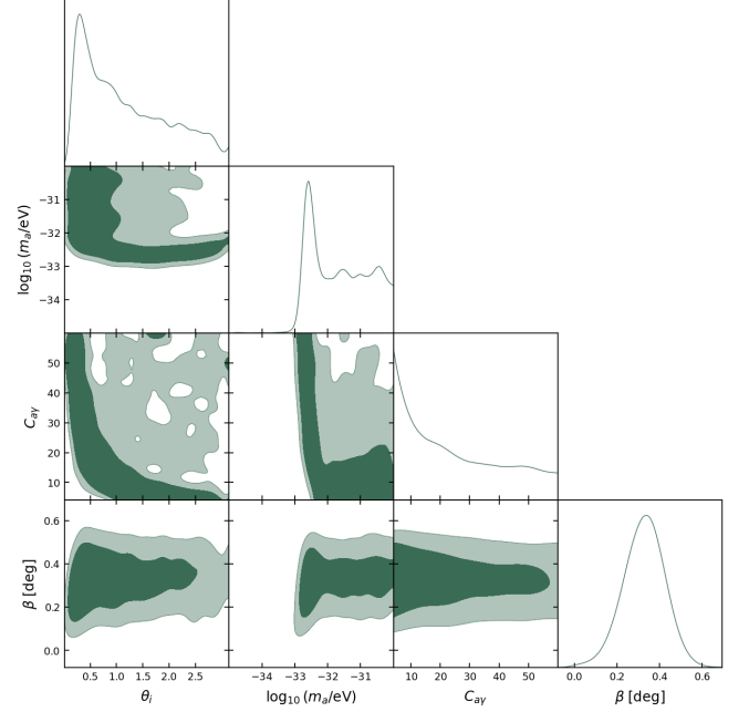
FIG. 4. Spectator-ALP joint posterior triangle from the continuous-prior cross-check configuration in which the photon anomaly coefficient is sampled freely (flat priors C_{a\gamma} \in [4, 60] — shifted and extended from the earlier [1, 30] to cover the posterior-supported coupling band (median 20.7, 16–84% [7.3, 45.6]); the dropped [1, 4] interval lies entirely below the minimum coupling \approx 8.6 required to reach the central value \beta = 0.342^\circ at the largest in-box displacement \Delta\phi/f_a = 1.19 — couplings in [4, 8.6] remain posterior-supported because the summary likelihood permits \beta below the central value — \theta_i \in [0.01, \pi] , \log_{10}(m_a/\text{eV}) \in [-35, -30] — the mass prior corresponds to m/H_0 \approx 7 \times 10^{-3} to 7 \times 10^2 for H_0 = 67.7 km/s/Mpc = 1.44 \times 10^{-33} eV), broadening the fixed- C_{a\gamma} = 8 and C_{a\gamma} \in [1, 30] configurations of Appendix C; the direct-sample priors are on the underlying ALP parameters ( \theta_i, m_a ), with \Delta\phi/f_a derived along each trajectory. The rotation marginal, \beta = 0.326^\circ \pm 0.099^\circ , is consistent within 1\sigma with the fixed- C_{a\gamma} = 8 result \beta_{\text{ALP}} = 0.336^\circ \pm 0.10^\circ and the observed \beta_{\text{obs}} = 0.342^\circ \pm 0.094^\circ (an internal-consistency statement: all three are constrained by the same single published \beta_{\text{obs}} , not independent measurements). The \theta_i - C_{a\gamma} anti-correlation band traces the constant-product degeneracy enforced by the summary-likelihood constraint through C_{a\gamma}(\Delta\phi/f_a) \approx 10.3 , and the m_a marginal piles toward the upper (heavier) edge of its prior range — the data-driven pull toward the upper edge of the natural-prior box discussed in the text, consistent with the model accommodating rather than naturally predicting the observed rotation (fn. 6).
