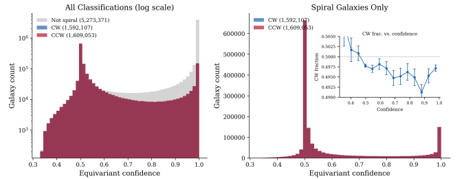
FIG. 6. Distribution of classifier confidence scores \max(\hat{p}_c) across all 8.47 million galaxies. The model assigns high confidence ( > 0.9 ) to 37.9% of predictions, indicating well-calibrated uncertainty for ambiguous morphologies.
