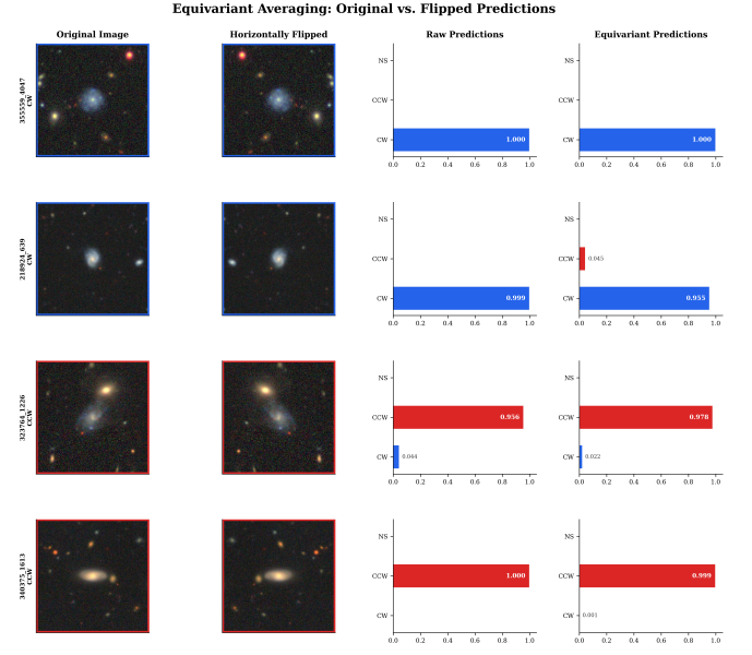
FIG. 4. Demonstration of the flip-equivariance consistency loss. For each galaxy image x , the model is trained to satisfy p_{\text{CW}}(x) \approx p_{\text{CCW}}(\mathcal{F}[x]) . The raw model achieves flip-swap correlation r = 0.833 ; test-time equivariant averaging (averaging predictions on the original and flipped image) recovers r = 1.000 exactly.
