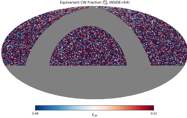
FIG. 13. Mollweide projection of the equivariant CW fraction f_{CW}^{eq} at N_{side} = 64 . No coherent large-scale pattern is visible.
