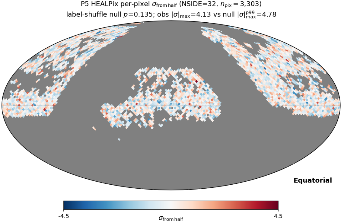
FIG. 4. Per-pixel signed \sigma_{\text{from half}} for the chirality-relevant matched-spiral subsample at NSIDE=32 (Mollweide projection, equatorial coordinates). The observed |\sigma|_{\text{max}}^{\text{obs}} = 4.13 vs the label-shuffle null |\sigma|_{\text{max}}^{\text{null}, p99} = 4.78 gives a look-elsewhere p = 0.135 ; no NSIDE returns p < 0.05 . The map shows no coherent large-scale structure beyond random pixel-level scatter; the high- |\sigma| pixels are isolated rather than clustered, consistent with the counting-statistics distribution expected from label-shuffle.
