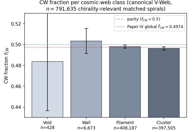
FIG. 3. CW fraction per cosmic-web class on the canonical V-Web run, on the n = 812,793 env-labeled spiral rows (covering 783,820 of the 791,635 unique chirality-relevant matched spirals; 7,815 lack an environment row, §VIA). Bars show the observed f_{\text{CW}} per class; black error bars are 95% Jeffreys binomial credible intervals, drawn on the row-level parent — the 2.7% duplicate rows violate strict i.i.d., but the worst-case design-effect inflation of the interval widths is \sqrt{812,793/783,820} = 1.018 , i.e. \leq 1.9\% , and the homogeneity \chi^2 is recomputed on the unique-spiral subset in §VIA. The void bin ( n = 428 ) is dominated by counting noise and brackets parity. The dashed horizontal line is parity ( f_{\text{CW}} = 0.5 ); the dotted red line is the Paper IV global \bar{f}_{\text{CW}} = 0.4974 classifier-monopole offset. All four classes bracket the Paper IV monopole, consistent with no environmental dependence beyond the catalog-wide classifier bias.
