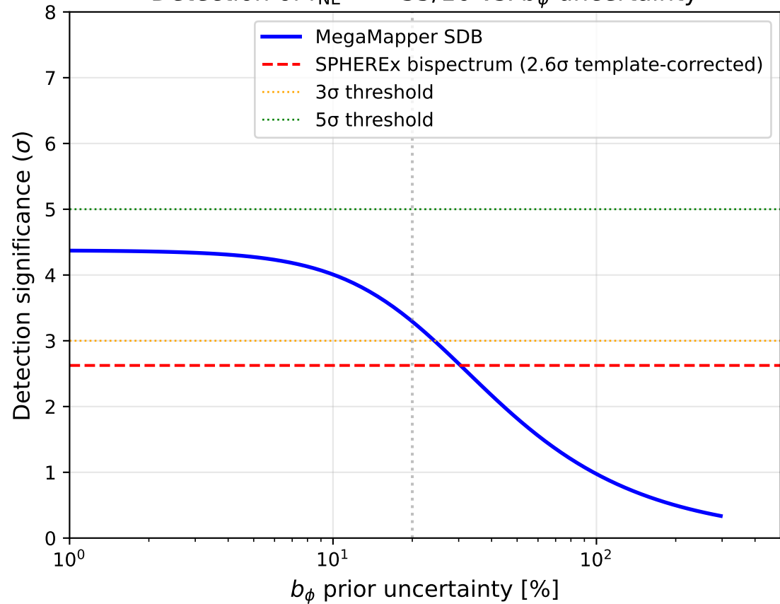
Detection of f_{\text{NL}} = -35/16 vs. b_\phi uncertainty
