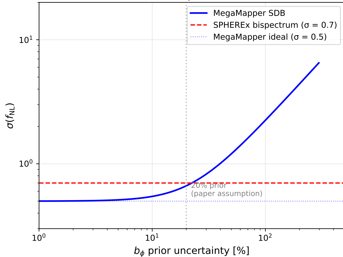
\sigma(f_{\text{NL}}) vs. b_\phi prior width
