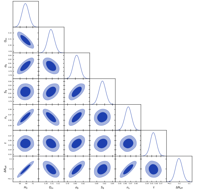
FIG. 3. Full-tension MCMC corner plot (119,617 post-burnin samples) over the joint Planck+BAO+SN+H0+ S_8 combination. Marginal posteriors for H_0 , \Omega_m , \sigma_8 , S_8 , and \Delta N_{\text{eff}} are shown on the diagonal; 2D contours at 1\sigma and 2\sigma levels off-diagonal. The \Delta N_{\text{eff}} posterior is consistent with zero ( -0.019 \pm 0.169 ), confirming that the spin-torsion framework does not inject additional relativistic species at recombination.
