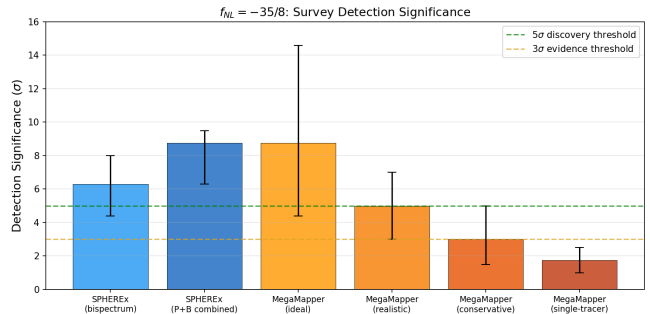
FIG. 2. Detection significance for f_{\text{NL}} = -35/8 across survey configurations. Error bars span the optimistic endpoint (published ideal \sigma(f_{\text{NL}}) with template-overlap correction only) to the conservative endpoint (full §VII budget: r = 0.84 overlap, \epsilon -correction, photometric- z degradation, PNG bias, b_\phi marginalization); i.e. optimistic-to-conservative ranges accounting for multi-tracer, photo- z , bias, and GR systematics.
