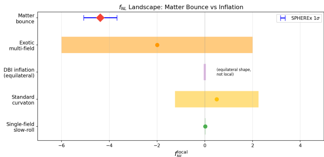
FIG. 3. f_{\text{NL}} landscape: matter bounce vs. inflationary alternatives. The bounce prediction (red diamond) is strongly constrained (minimally parameterized); inflationary alternatives require additional free parameters to reach the same region. SPHEREx 1\sigma error bar shown in blue.
