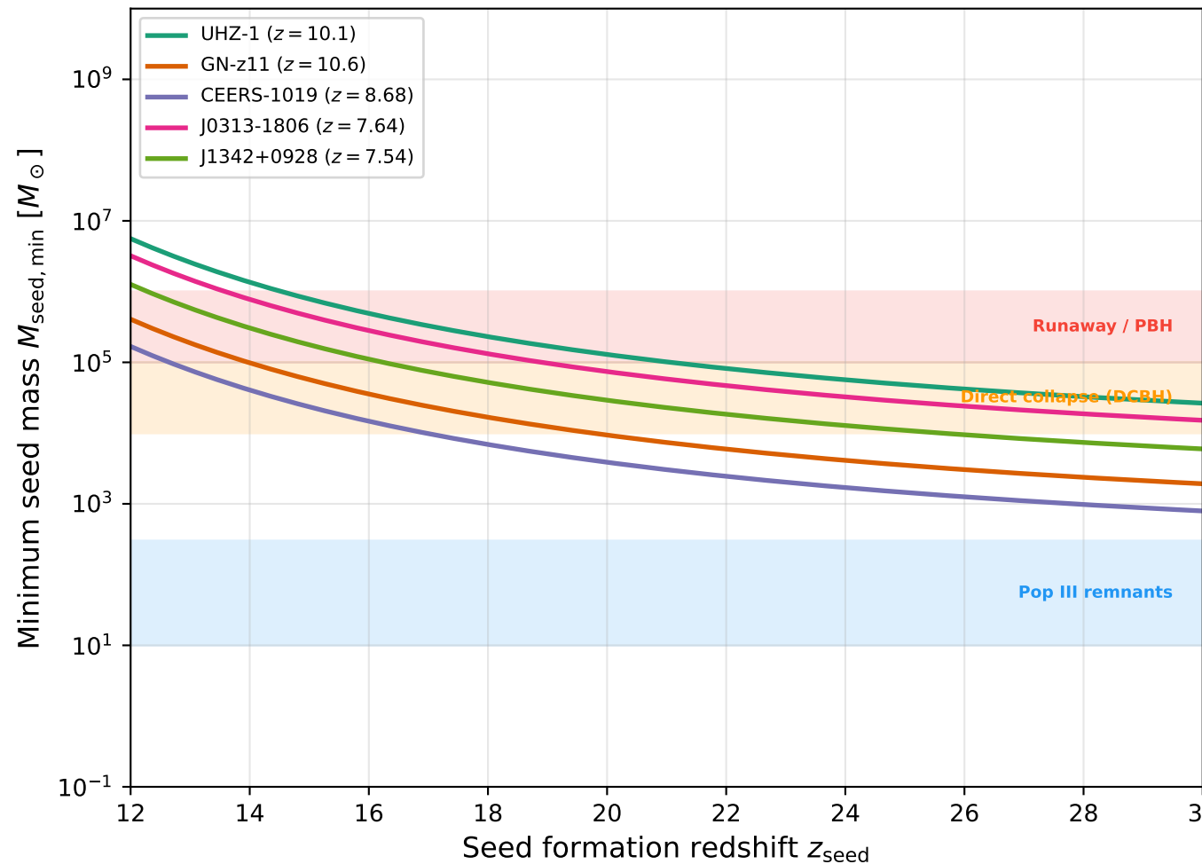
Planck 2018
