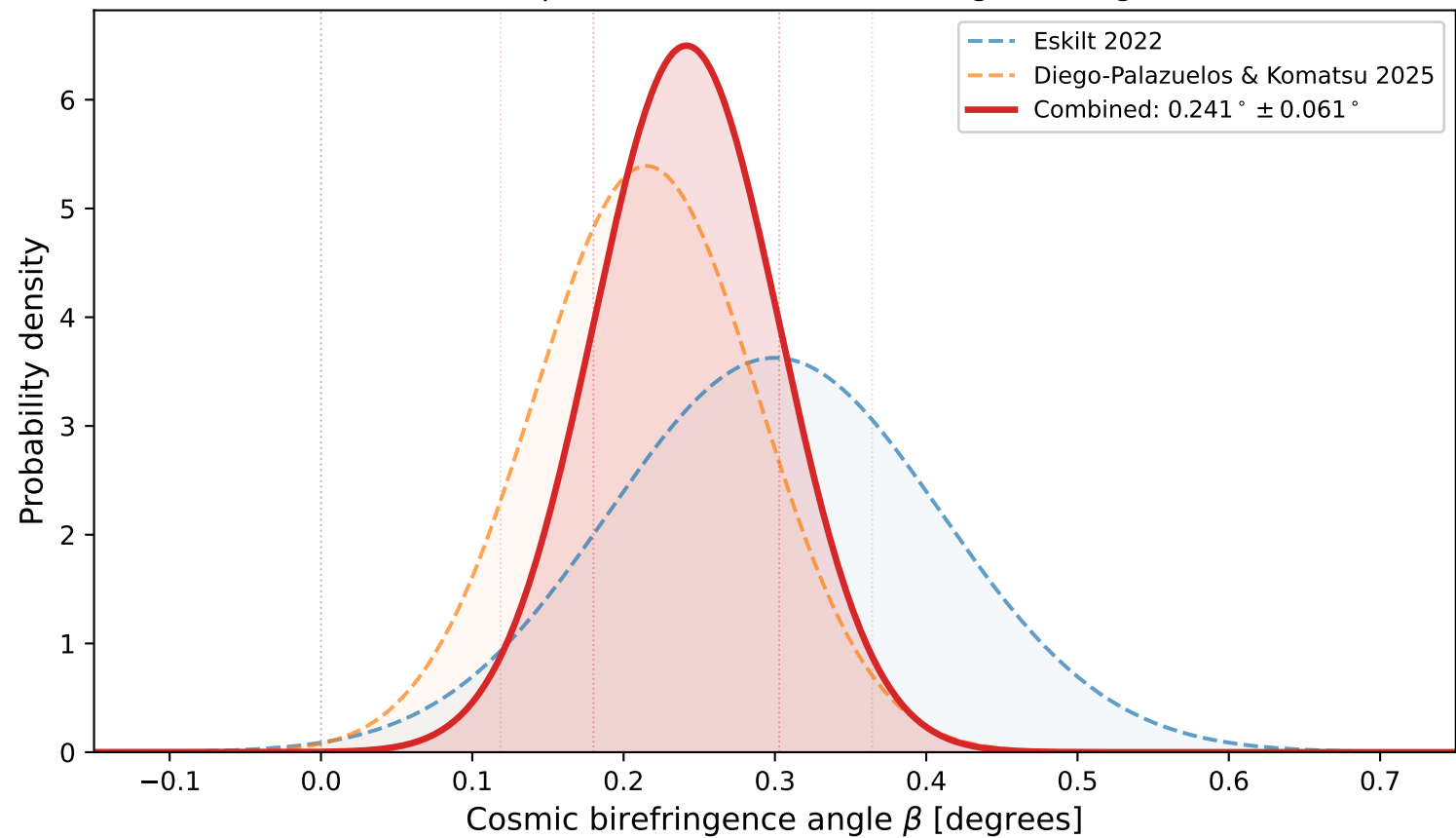
Gaussian posterior on cosmic birefringence angle
