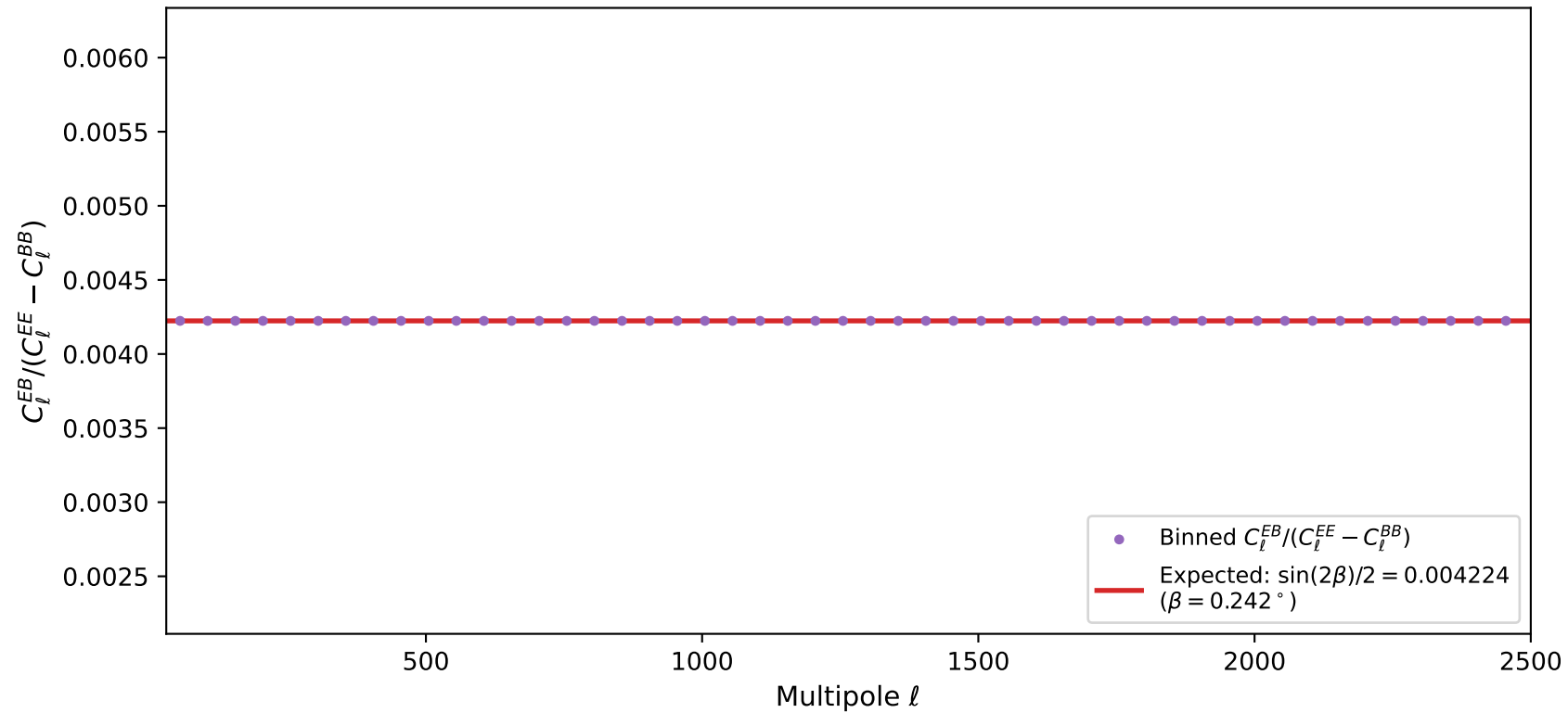
Isotropy diagnostic: ratio should be constant for isotropic birefringence
