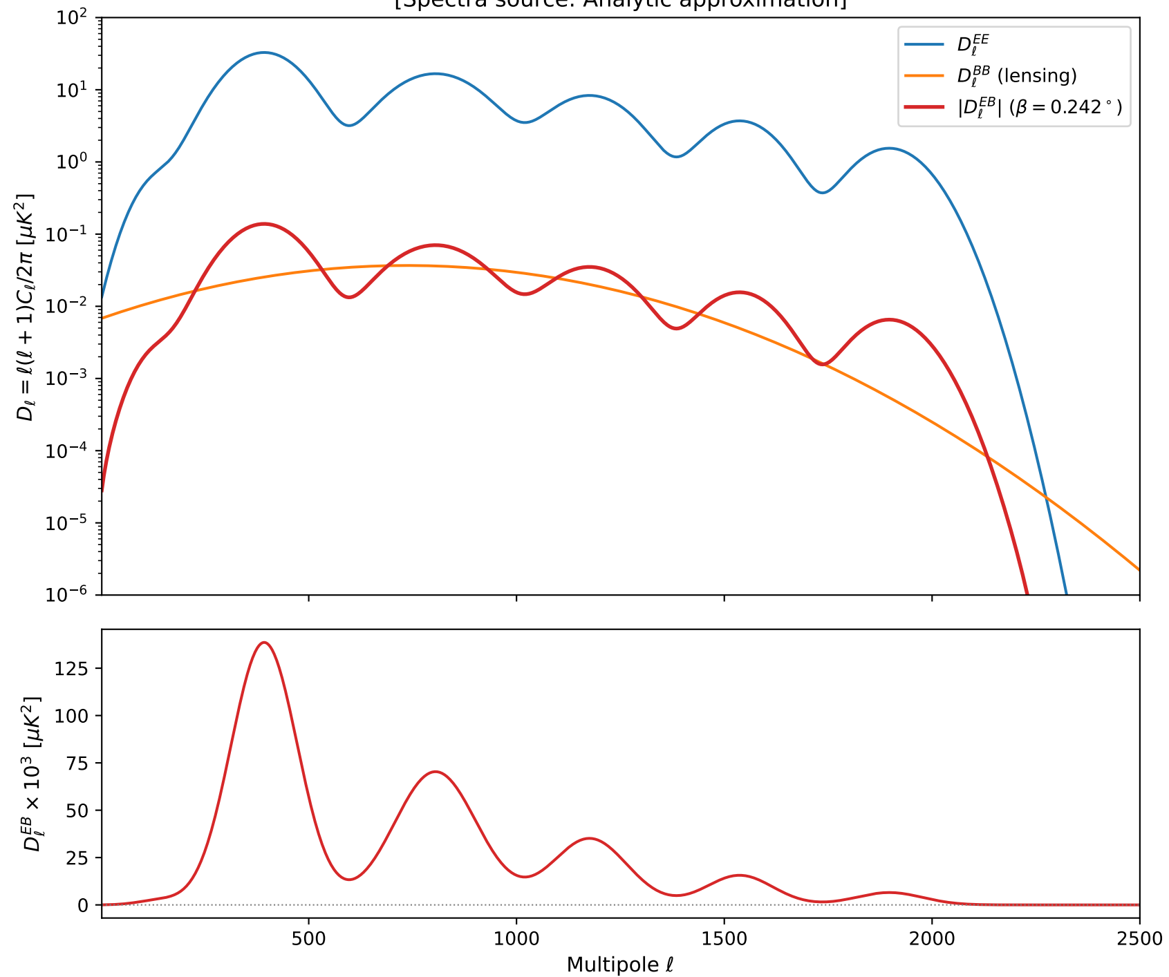
Predicted EB spectrum from isotropic birefringence [Spectra source: Analytic approximation]
