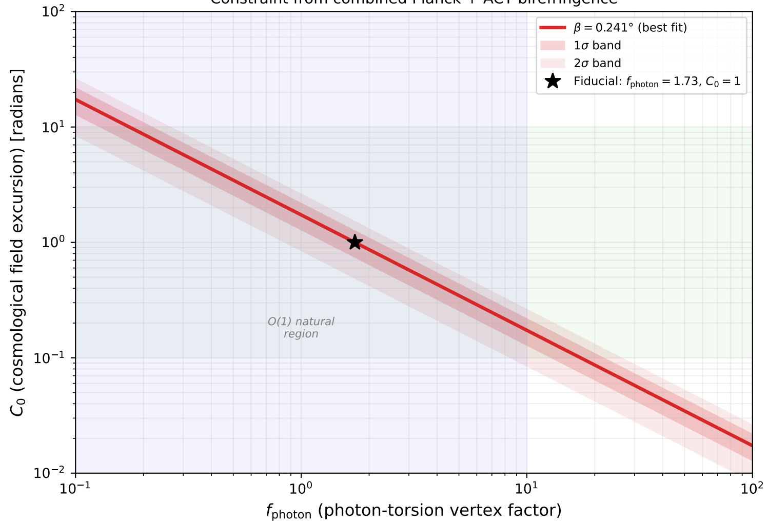
Degeneracy: \beta = \varepsilon \cdot f_{\text{photon}} \cdot C_0 Constraint from combined Planck + ACT birefringence
