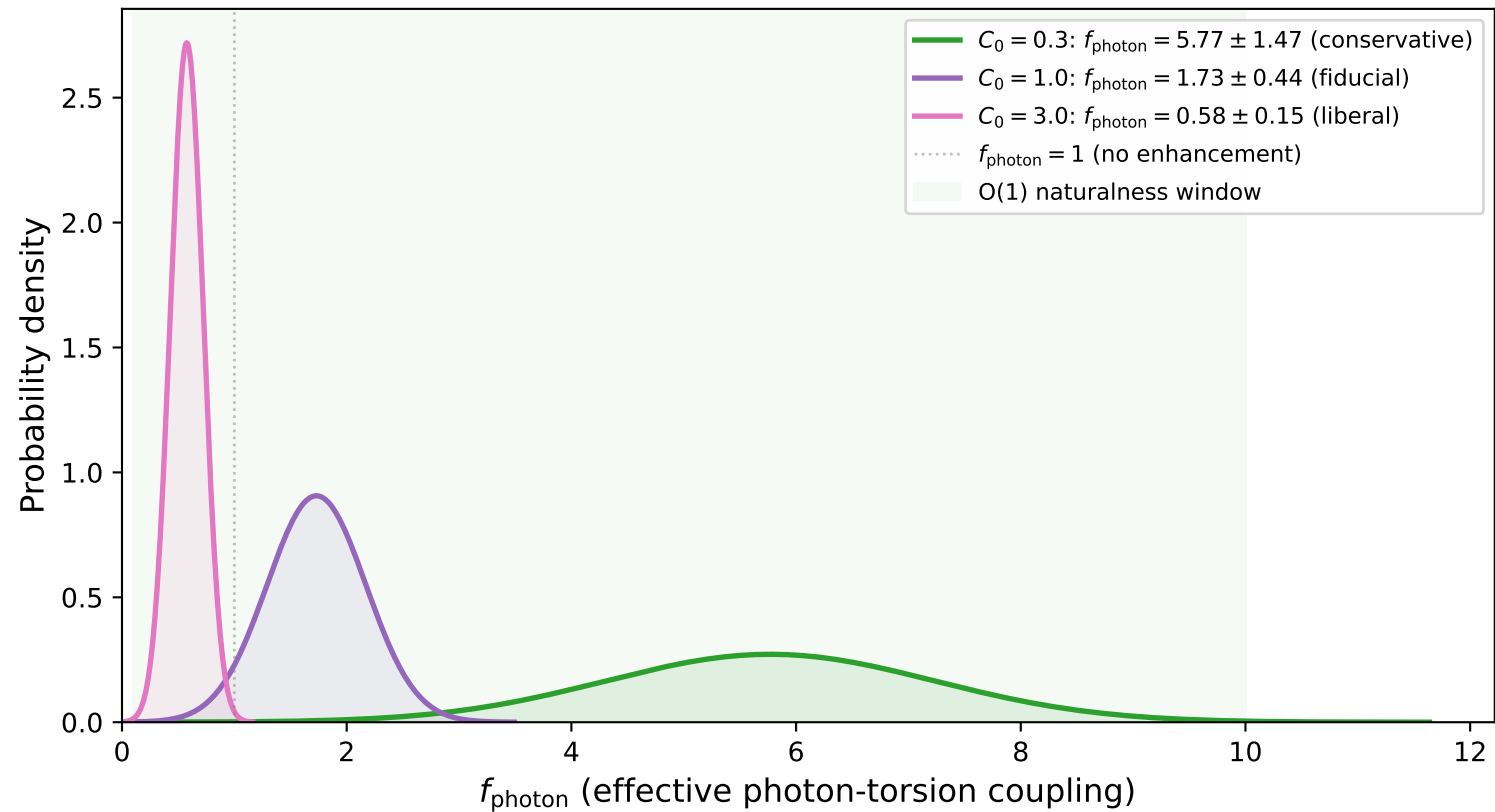
Derived posterior on f_{\text{photon}} ( \varepsilon = (\alpha/M) M_{\text{Pl}} = 2.435e-03 )
