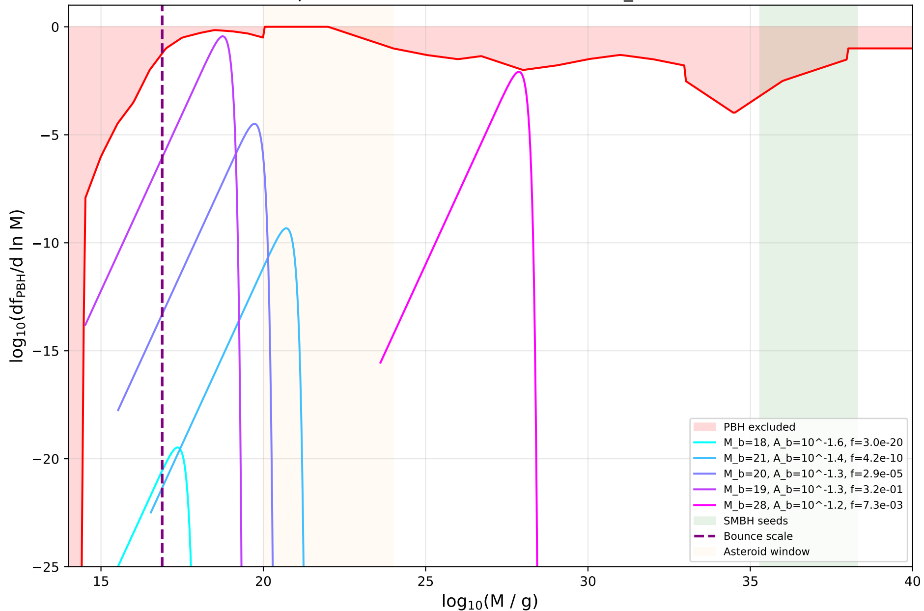
Representative PBH Mass Functions ( s_k = 0.3 )
