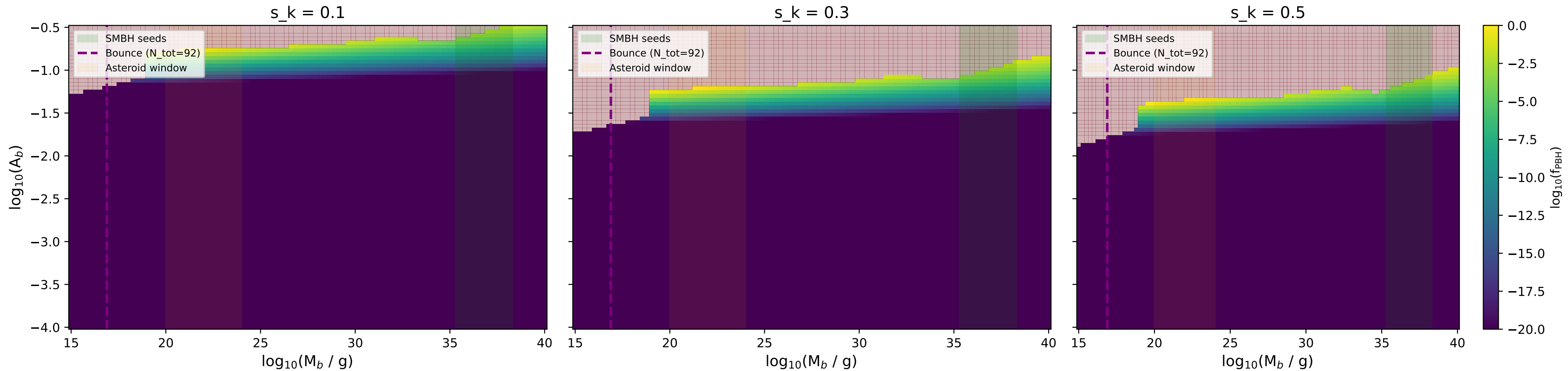
Chain 1A: PBH Viability Map (colored = viable, red = excluded by PBH bounds)
