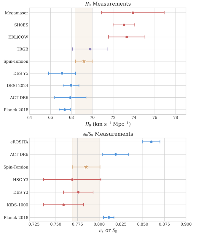
FIG. 6. MCMC fits compared with nine published measurements against nine published measurements. Top panel: H_0 measurements from Planck (early universe), ACT DR6, DESI BAO, DES Y5, our spin-torsion model, H0LiCOW, SH0ES, Megamaser Project, and TRGB. Bottom panel: \sigma_8/S_8 measurements including Planck, KiDS-1000, DES Y3, HSC Y3, eROSITA, and ACT DR6.
