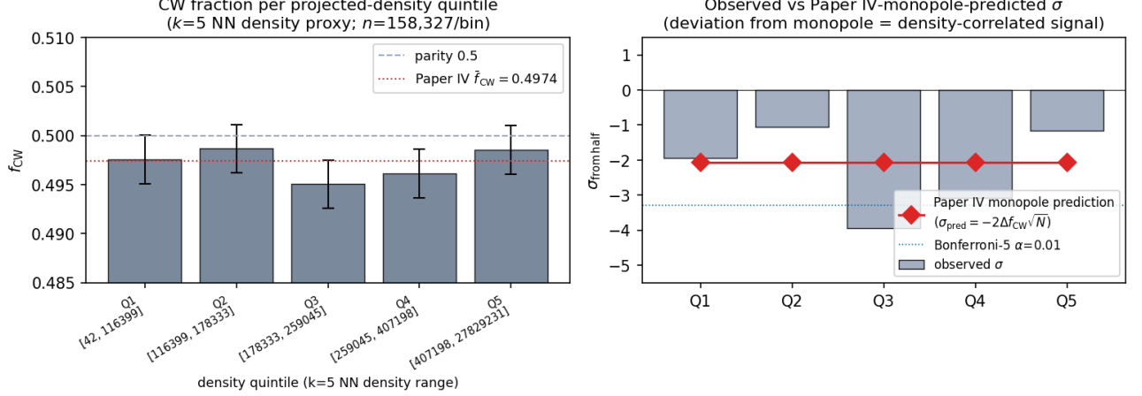
FIG. 5. Density-quintile null with Paper IV monopole-prediction overlay. Left : CW fraction per projected-density quintile ( k=5 NN proxy, N=158,327 per bin) with 95% Jeffreys binomial CIs; dashed parity f_{CW}=0.5 and dotted Paper IV \bar{f}_{CW}=0.4974 references. Right : observed \sigma_{\text{from half}} per quintile (bars) vs the Paper IV-monopole prediction \sigma_{\text{pred}}=2\Delta f_{CW}\sqrt{N} (red diamonds) at \Delta f_{CW}=-0.0026 ; dotted blue lines mark the Bonferroni-5 thresholds at \alpha=0.01 . The observed signed \sigma tracks the monopole prediction within counting statistics; no quintile deviates from the prediction by more than \sim 2\sigma .
