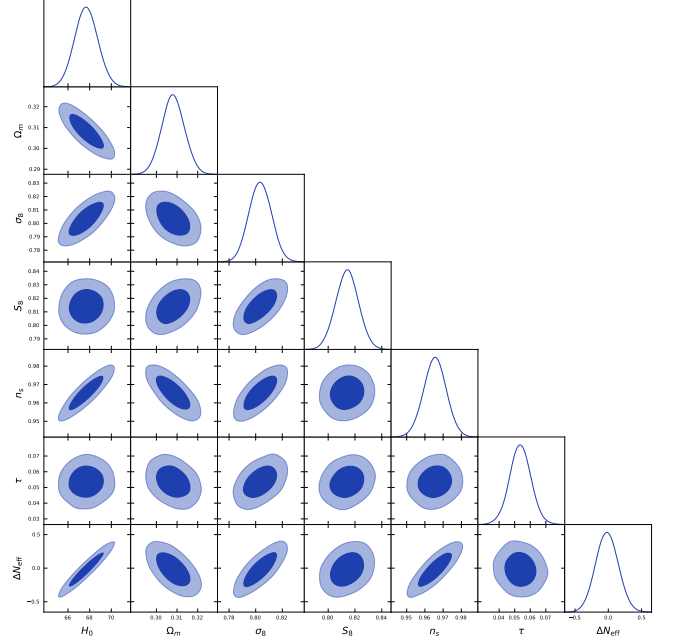
FIG. 4. Full-tension MCMC corner plot (119,617 post-burnin samples, a getdist -thinned slice of the 176,840 raw samples reported in Table II; see footnote 4) over the joint Planck+BAO+SN+H0+ S_8 combination. Marginal posteriors for H_0 , \Omega_m , \sigma_8 , S_8 , and \Delta N_{\text{eff}} are shown on the diagonal; 2D contours at 1\sigma and 2\sigma levels off-diagonal. The \Delta N_{\text{eff}} posterior is consistent with zero ( -0.020 \pm 0.169 ), confirming that the spin-torsion framework does not inject additional relativistic species at recombination.
