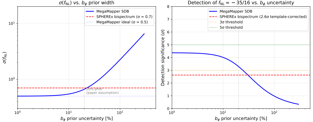
FIG. 5. Left: \sigma(f_{\text{NL}}) as a function of b_\phi prior uncertainty for MegaMapper SDB (blue). The SPHEREx bispectrum constraint (red dashed) is less sensitive to b_\phi but not independent of it; the residual dependence enters at tree level through the \Delta b(k) \propto f_{\text{NL}} b_\phi / k^2 cross-terms f_{\text{NL}} b_\phi b_1^2 P(k_1) P(k_2) in the multi-tracer Fisher matrix [3], which propagate to all triangle configurations and not only the squeezed limit. Right: corresponding detection significance for the corrected central f_{\text{NL}} = -35/16 (all significances one-half of the erroneous -35/8 values). At the paper’s assumed 20% prior (gray line; the SPHEREx multi-tracer bispectrum combined-sample baseline is \sigma(f_{\text{NL}}) = 0.7 at this point, not a per-redshift-bin uncertainty), MegaMapper gives \sim 2\sigma ; relaxing the per-tracer-bin b_\phi prior to 30% widens the combined-sample SPHEREx \sigma(f_{\text{NL}}) to \approx 0.9 – 1.0 , and relaxing to 50% drops MegaMapper to \sim 1\sigma . The bispectrum channel remains at \sim 2.6\sigma (optimistic) or \sim 1.5 – 2\sigma (after GR degradation) at fixed Heinrich et al. b_\phi universality [3]; relaxing b_\phi universality per tracer bin [35] degrades the optimistic 2.6–2.75 \sigma headline to \sim 2.0 – 2.1\sigma (30% central) and \sim 1.75 – 1.85\sigma (50% conservative).
