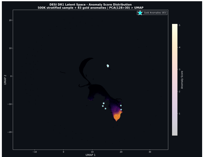
Figure 1. 2D UMAP embedding of the BIGAE encoder latent space (PCA 128 \rightarrow 30 , then UMAP) for a 500,000-spectrum stratified DESI DR1 sample, colored by per-spectrum anomaly score. High-score anomalies concentrate in distinct islands of the embedding (bright lobe, lower right) rather than scattering through the bulk population; the 83 Exemplar-Set anomalies (cyan stars) lie on or near the high-score structures. The 83-object Exemplar Set is a display-only, ranked visual sample of the companion high- z candidate pipeline (force-included in the embedding; not a catalog tier and not a density-representative sample; §3.2).
