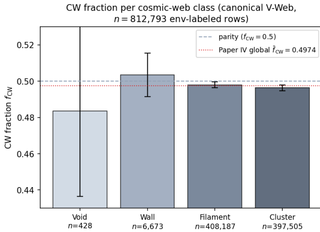
FIG. 3. CW fraction per cosmic-web class on the headline V-Web run, on the n = 812,793 env-labeled spiral rows (covering 783,820 of the 791,635 unique chirality-relevant matched spirals; 7,815 lack an environment row, §VI A). Bars show the raw observed f_{CW} per class (counts shown; monopole subtraction enters the \sigma_{vs\text{ monopole}} column only); black error bars are 95% Jeffreys binomial credible intervals, drawn on the row-level parent — the 3.56% duplicate rows (28,973 of 812,793 env-labeled rows) violate strict i.i.d., but the worst-case design-effect inflation of the interval widths is \sqrt{812,793/783,820} = 1.018 , i.e. \leq 1.9\% , and the homogeneity \chi^2 is recomputed on the unique-spiral subset in §VI A. The void bin ( n=428 ) is dominated by counting noise and brackets parity. The dashed horizontal line is parity ( f_{CW} = 0.5 ); the dotted red line is the Paper IV global \bar{f}_{CW} = 0.4974 classifier-monopole offset. All four classes bracket the Paper IV monopole, consistent with no environmental dependence beyond the catalog-wide classifier bias.
