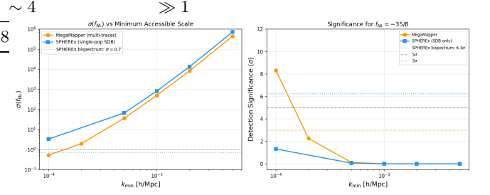
FIG. 4. Left: \sigma(f_{\text{NL}}) vs. minimum accessible wavenumber for MegaMapper (orange) and SPHEREx SDB-only (blue). The SPHEREx bispectrum channel ( \sigma = 0.7 , dotted) avoids the ultra-large-scale fragility. Right: corresponding detection significance for f_{\text{NL}} = -35/8 .
