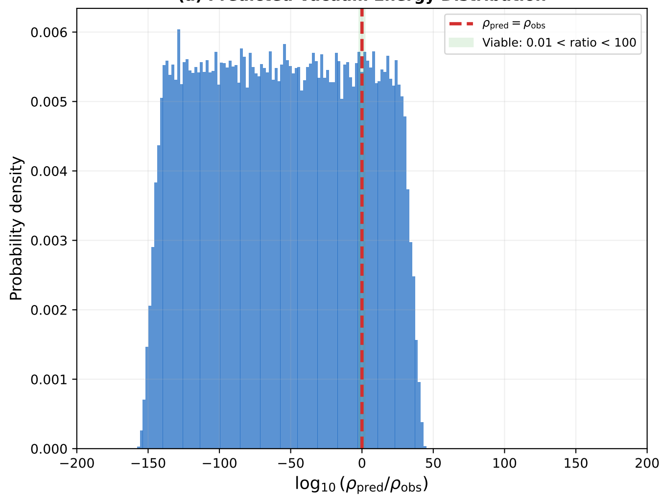
(a) Predicted Vacuum Energy Distribution
