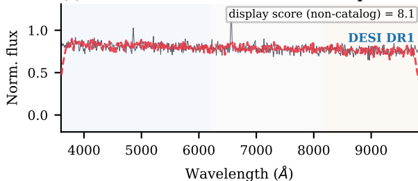
(e) Match 3: BAL QSO candidate — DESI
