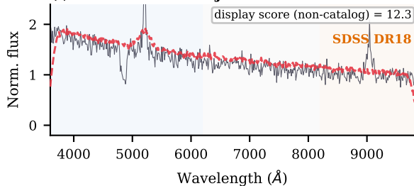
(f) Match 3: same object in SDSS
