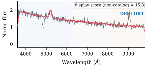
(e) Match 3: BAL QSO candidate — DESI
