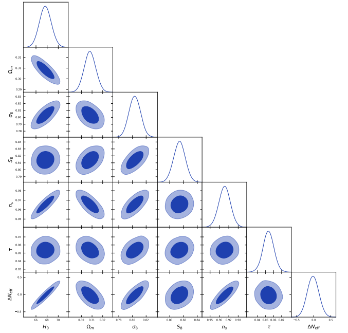
FIG. 4. Full-tension MCMC corner plot (119,617 post-burnin samples, a getdist -thinned slice of the 176,840 raw samples reported in Table II; see footnote 4) over the joint Planck+BAO+SN+ H_0 + S_8 combination. Marginal posteriors for H_0 , \Omega_m , \sigma_8 , S_8 , and \Delta N_{\text{eff}} are shown on the diagonal; 2D contours at 1\sigma and 2\sigma levels off-diagonal. The \Delta N_{\text{eff}} posterior is consistent with zero ( -0.020 \pm 0.169 ), confirming that the spin-torsion framework does not inject additional relativistic species at recombination.
