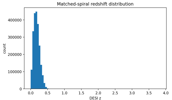
FIG. 1. Redshift distribution of the matched chirality \times DESI DR1 spiral sample (1'' acceptance, after dedup). The distribution peaks at z \approx 0.15 –0.2 (median 0.168) and falls off steeply above z \approx 0.5 ; a sparse tail extends to the maximum z = 3.83 (Table II).
