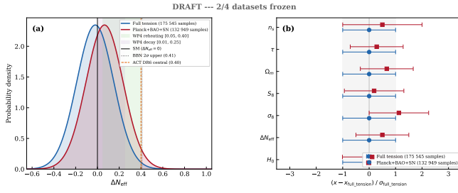
FIG. 4. \Delta N_{\text{eff}} posteriors from the two frozen verification datasets. Left : Gaussian approximations to the posteriors, with vertical lines marking the SM value ( \Delta N_{\text{eff}} = 0 ), BBN upper limit, and ACT DR6 central value. Shaded regions show the WP4 theory-predicted ranges from spin-torsion reheating and decay mechanisms. Right : Normalized parameter shifts between the two datasets, in units of the full-tension standard deviation.
