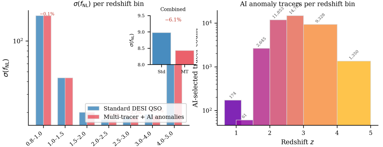
FIG. 9. Legacy fixed- \alpha reference — superseded by the empirical \alpha_{jk} result of §V. Per-redshift-bin decomposition of the fixed- \alpha = 0.15 reference Fisher forecast (Appendix C). Left: \sigma(f_{\text{NL}}) per redshift bin for the standard DESI QSO single-tracer baseline versus the multi-tracer configuration including AI-selected anomaly tracers; the inset shows the combined result ( \sigma(f_{\text{NL}})^{\text{std}} = 8.98 \rightarrow 8.43 , a 6.1% central-value change). Right: AI-selected anomaly-tracer counts per redshift bin; the seven bins total 40,192 tracers — the redshift-binned DESI anomaly subsample over 0.8 < z < 5.0 used as the additional tracer population in the reference Fisher configuration, distinct from both the full 195,829-object DESI anomaly catalog and the 5,384-object QSO-candidate bias sample of §V. This figure illustrates the fixed- \alpha reference configuration only; the primary forecast uses the empirical \alpha_{jk} = 0.19 \pm 0.65 ( \sigma(f_{\text{NL}}) = 8.14 central, 1\sigma envelope [3.92, 8.98] ), and in both cases the central improvement is consistent with no improvement at < 1\sigma — no positive multi-tracer detection is claimed.
