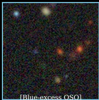
[Blue-excess QSO] RA 211.3° | AE=9240
