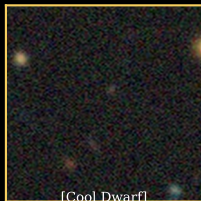
[Cool Dwarf] RA 175.9° | AE=4058
