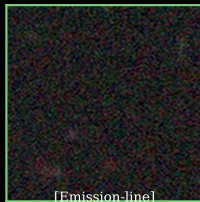
[Emission-line] RA 246.3° | AE=8280
