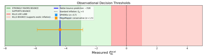
FIG. 6. Observational decision thresholds. Green: strongly favors bounce. Red: strongly disfavors the quasi-dust matter bounce. Blue vertical line: bounce prediction f_{\text{NL}} = -35/8 . Error bars: SPHEREx ( \sigma = 0.7 ) and MegaMapper conservative ( \sigma = 1.5 ).
