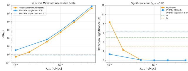
FIG. 4. Left: \sigma(f_{\text{NL}}) vs. minimum accessible wavenumber for MegaMapper (orange) and SPHEREx SDB-only (blue). The SPHEREx bispectrum channel ( \sigma = 0.7 , dotted) is less sensitive to the ultra-large-scale fragility. Right: corresponding detection significance for f_{\text{NL}} = -35/8 .
