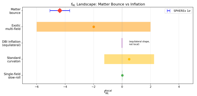
FIG. 3. f_{\text{NL}} landscape: matter bounce vs. inflationary alternatives. The bounce prediction (red diamond) is parameter-free; inflationary alternatives require free parameters to reach the same region. SPHEREx 1\sigma error bar shown in blue.
