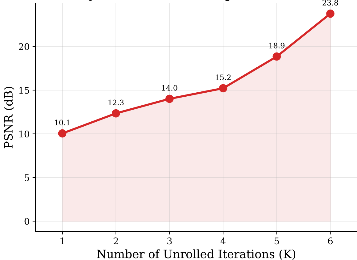
Model-Based JSCC: Iteration Convergence (SNR=10dB, Kodak)
