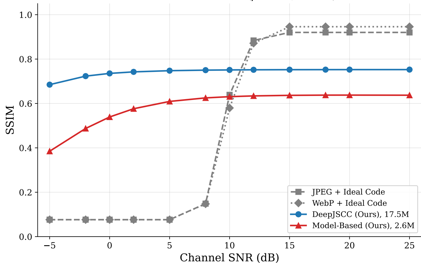
SSIM vs Channel SNR ( \rho = 1/4 , Kodak)
