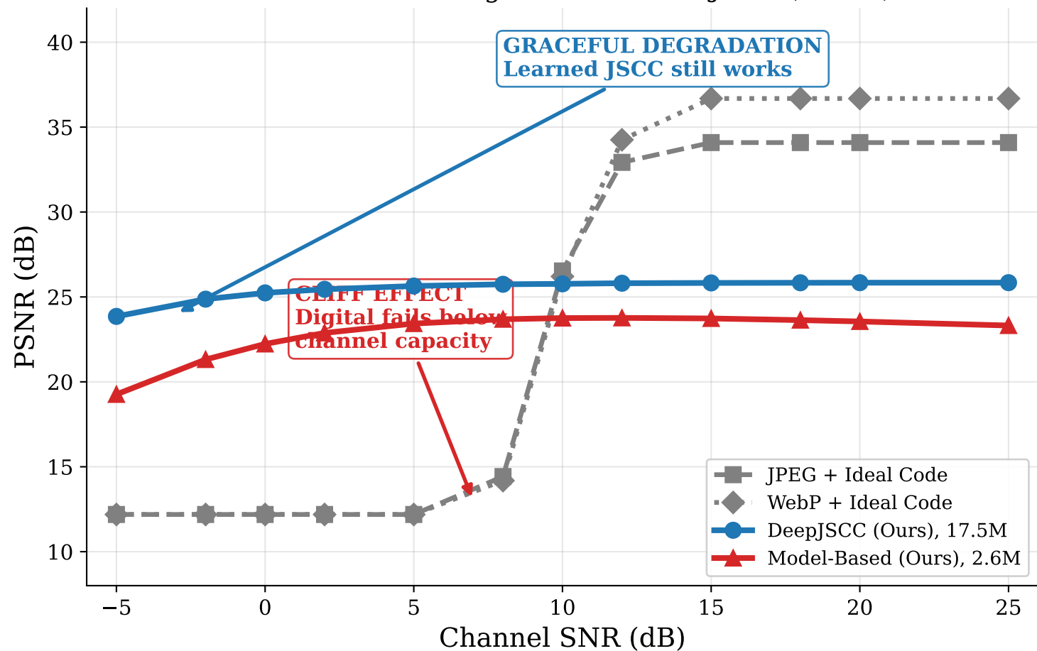
The Cliff Effect: Digital vs Learned JSCC (Kodak)
