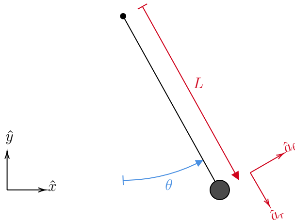
Figure 3.5: Pendulum Set-Up
