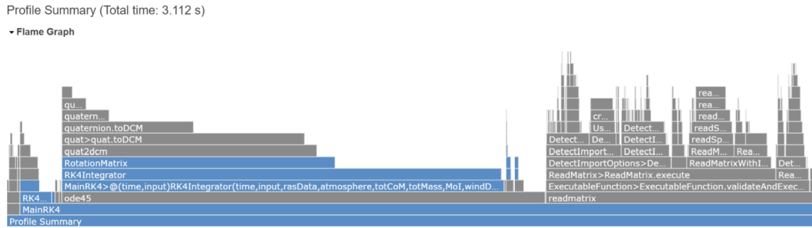
Figure 6.6: Flame Graph After Optimizations
