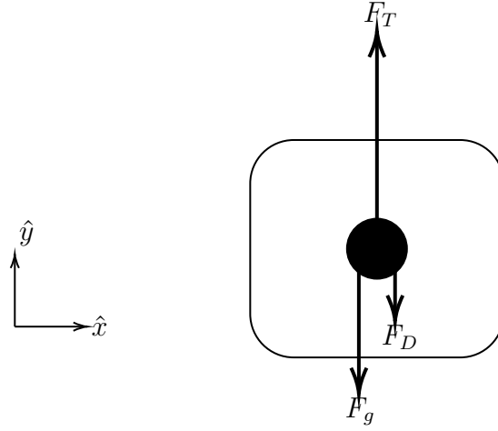
Figure 2.1: 1-DoF Forces on a body
