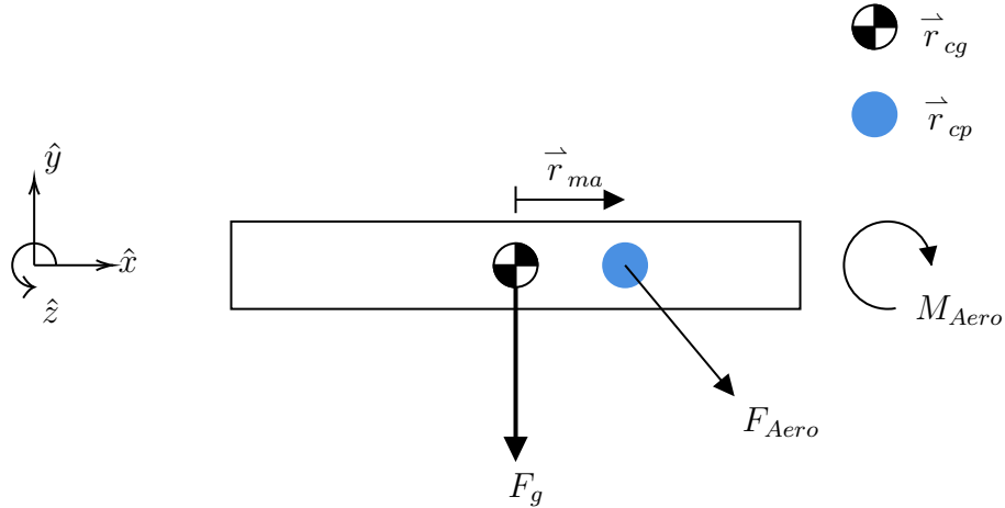
Figure 2.10: Moment Demonstration
