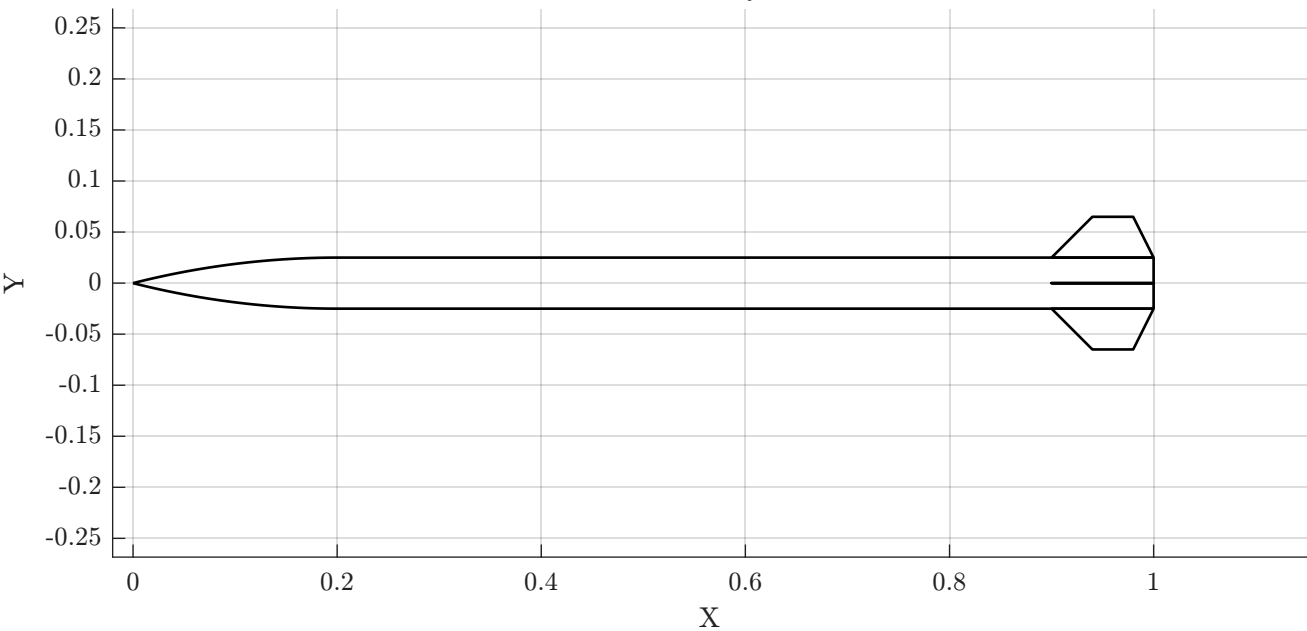
Rocket Layout
