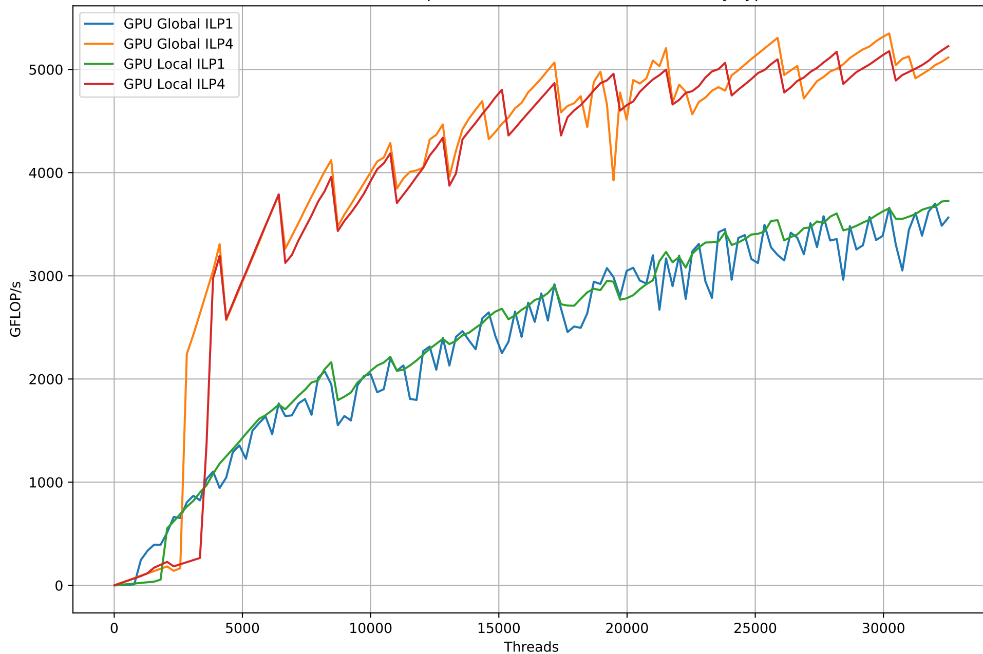
Performance Comparison of Different ILPs and Memory Types
