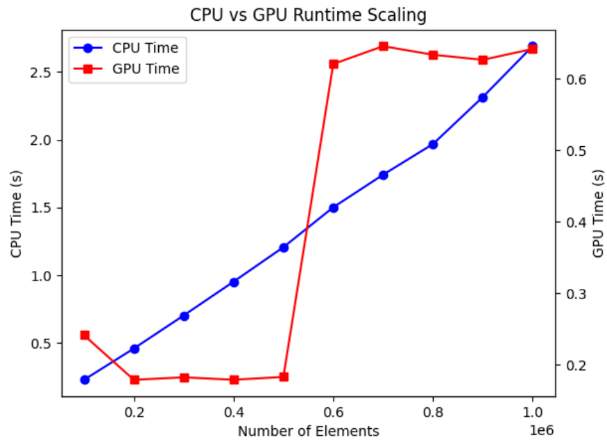
Figure 1: Execution times of the CPU and GPU scan algorithm for different number of elements. (Note: the y-axis are different for CPU and GPU)
