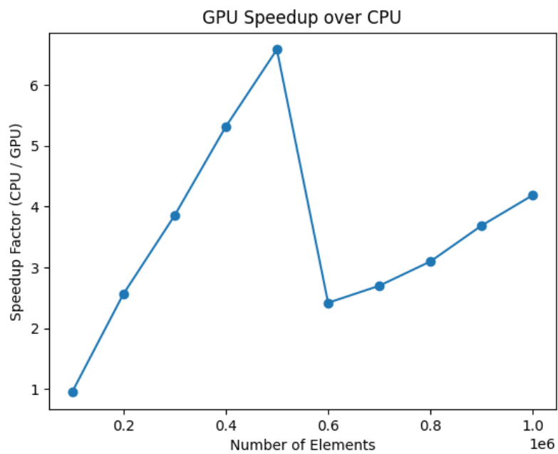
Figure 2: Speedup-Factor CPU/GPU of the scan algorithm for different number of elements
