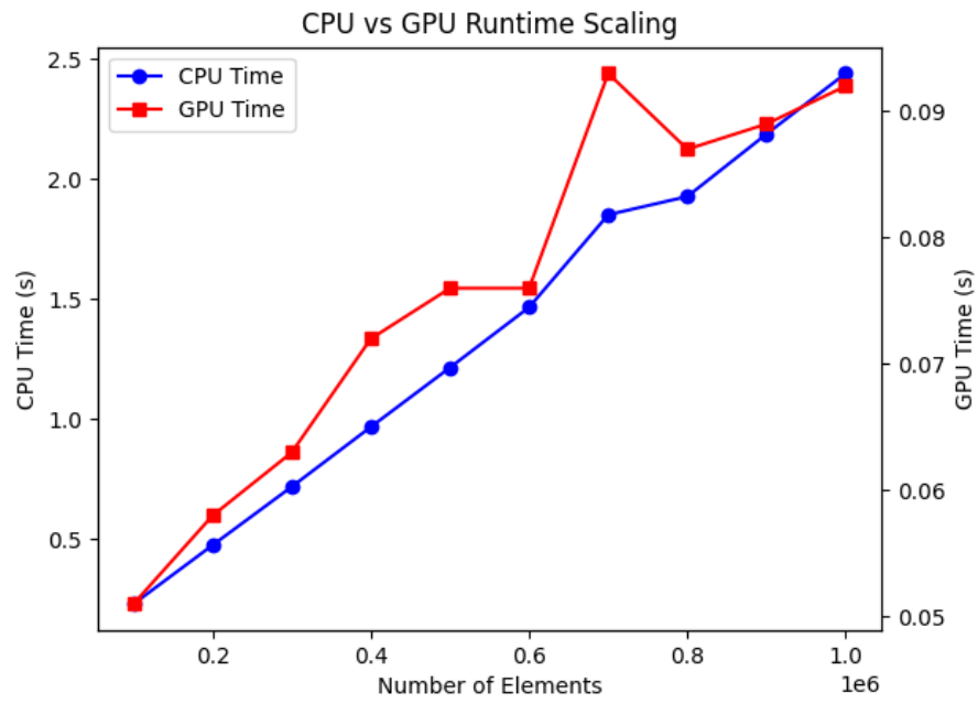
Figure 1: Execution times of the CPU and GPU scan algorithm for different number of elements. (Note: the y-axis are different for CPU and GPU)
