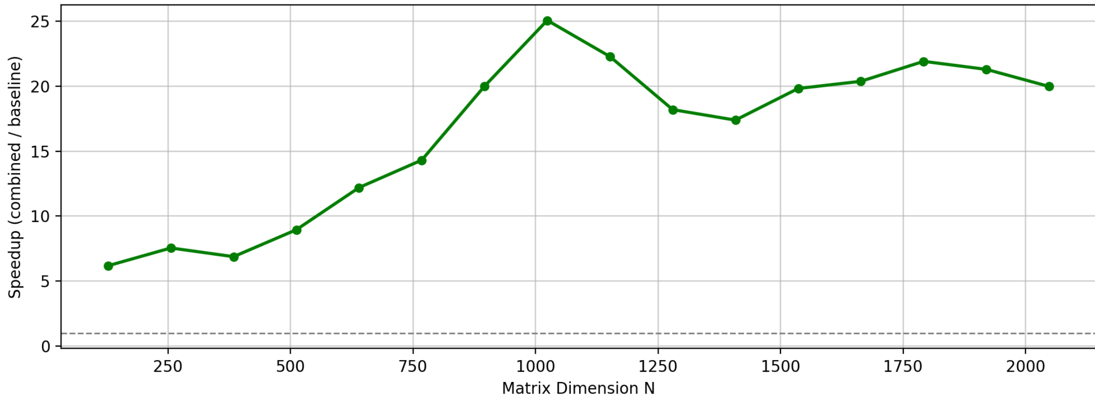
Part II - Speedup of combined method over -O3 baseline
