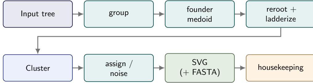
Figure 1: High-level data flow of tree_clustering.py (default path). With --as-is , the founder medoid and reroot + ladderize stages are skipped.
