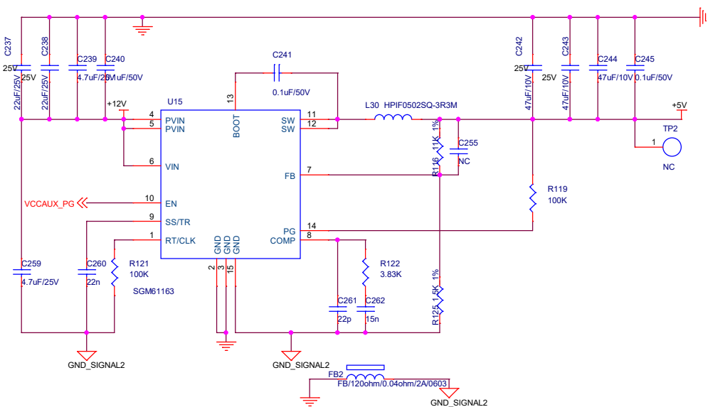
+5V POWER 6A
