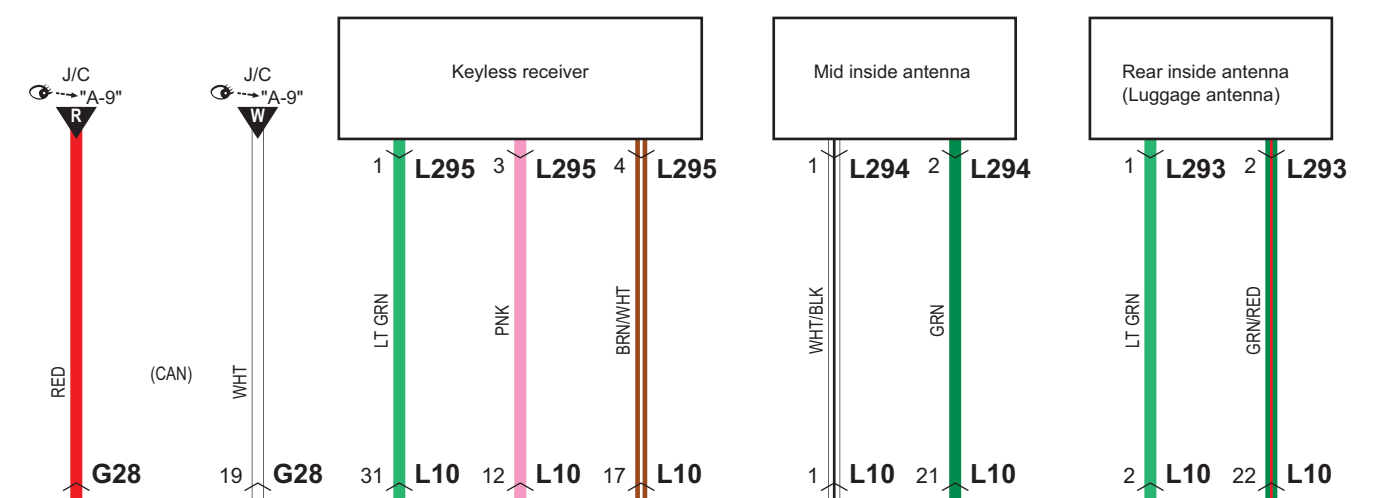
Keyless start control module
