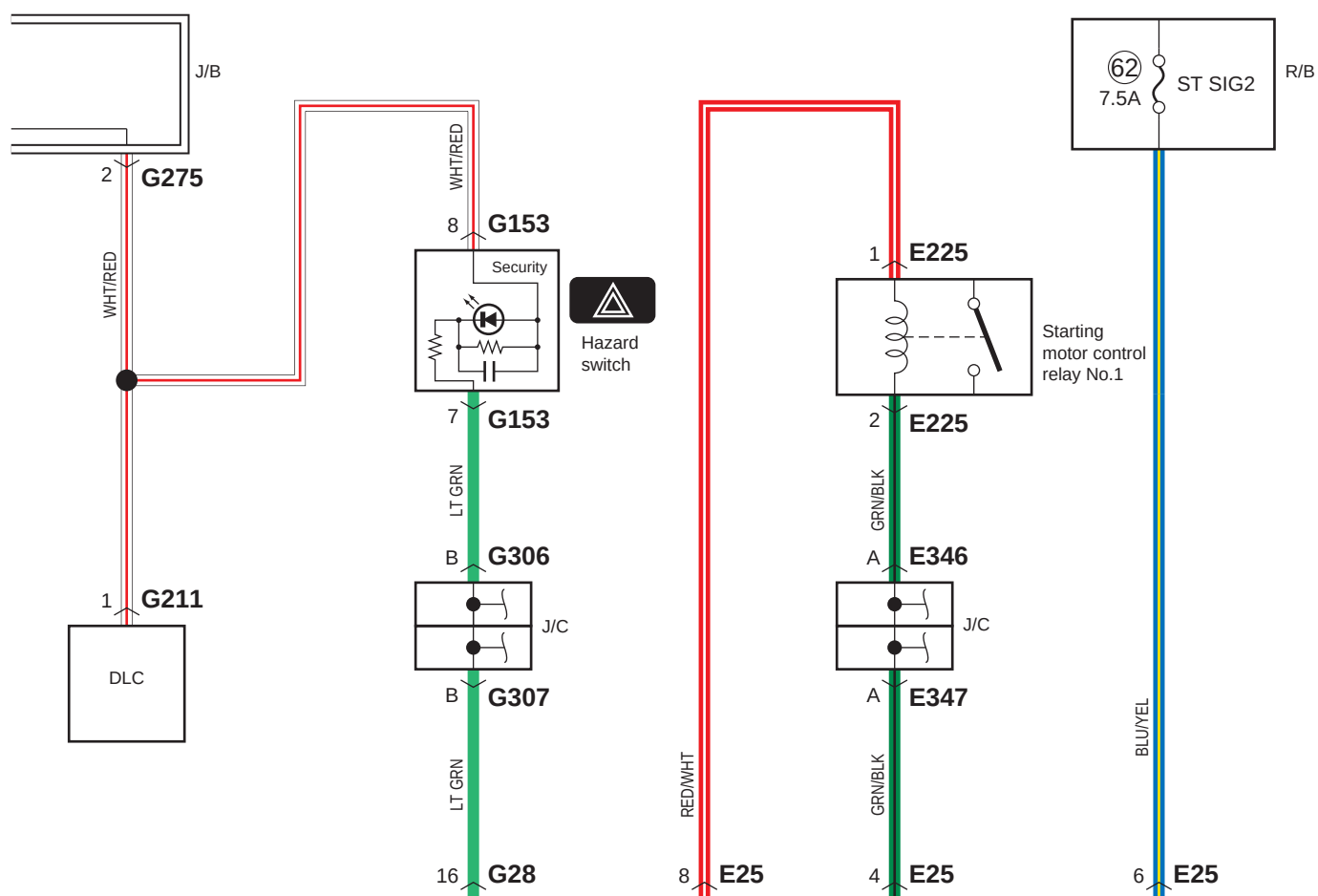
Keyless start control module
