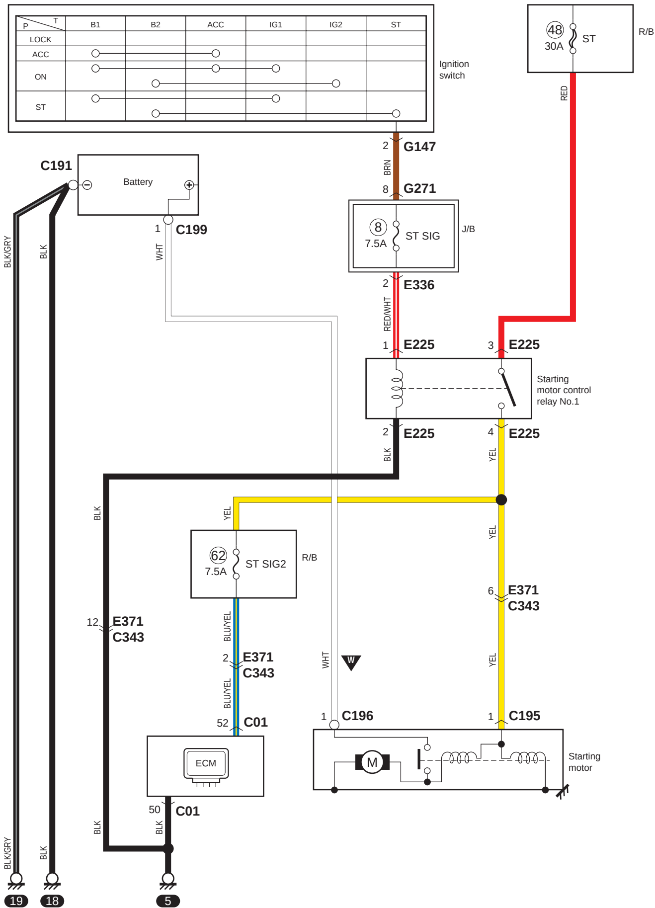
A-1-1 Cranking System Circuit Diagram (Petrol Model without Engine Push Start System)
