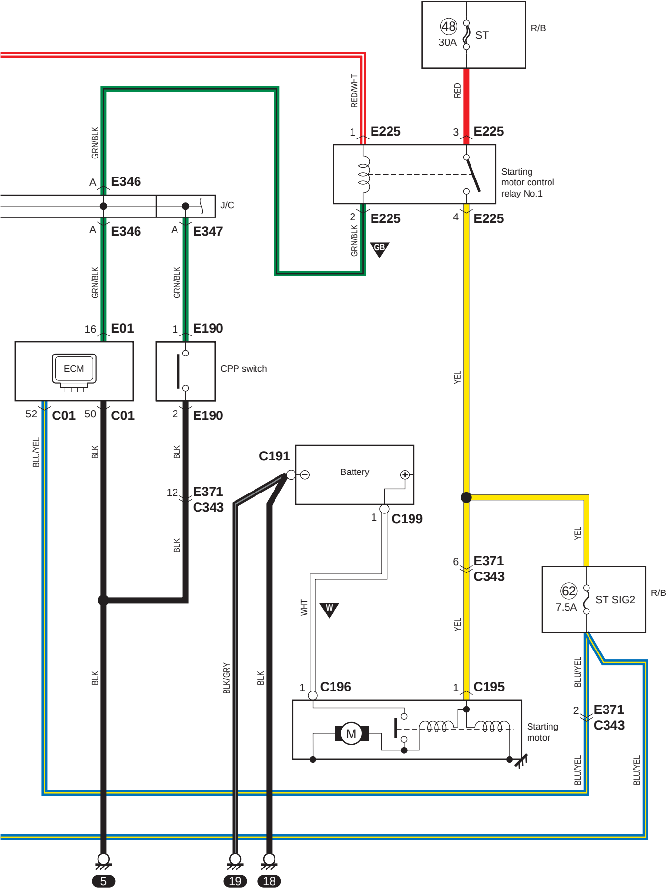
A-1-2 Cranking System Circuit Diagram (Petrol Model with Engine Push Start System)
