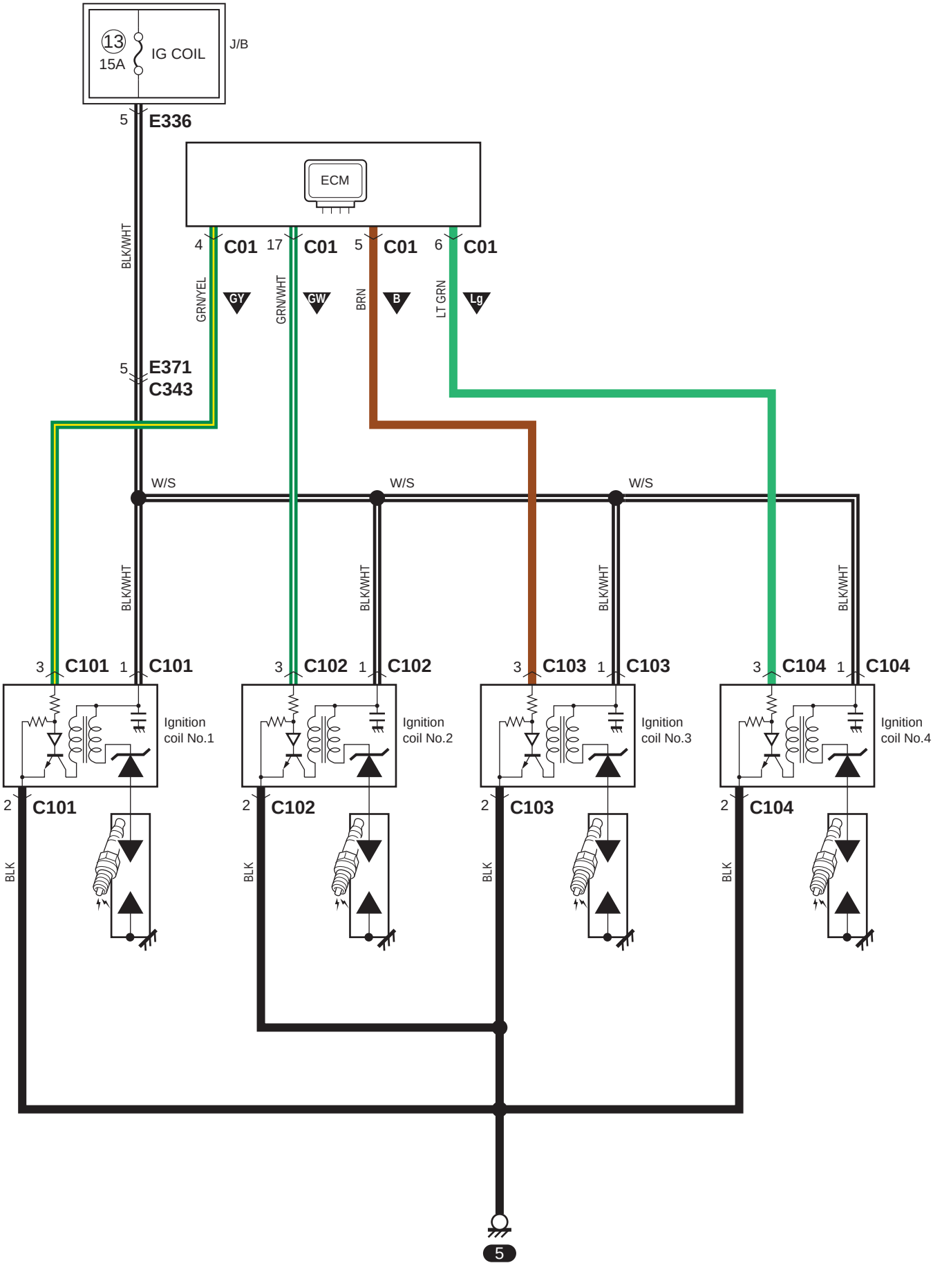
A-3 Ignition System Circuit Diagram (Petrol Model)
