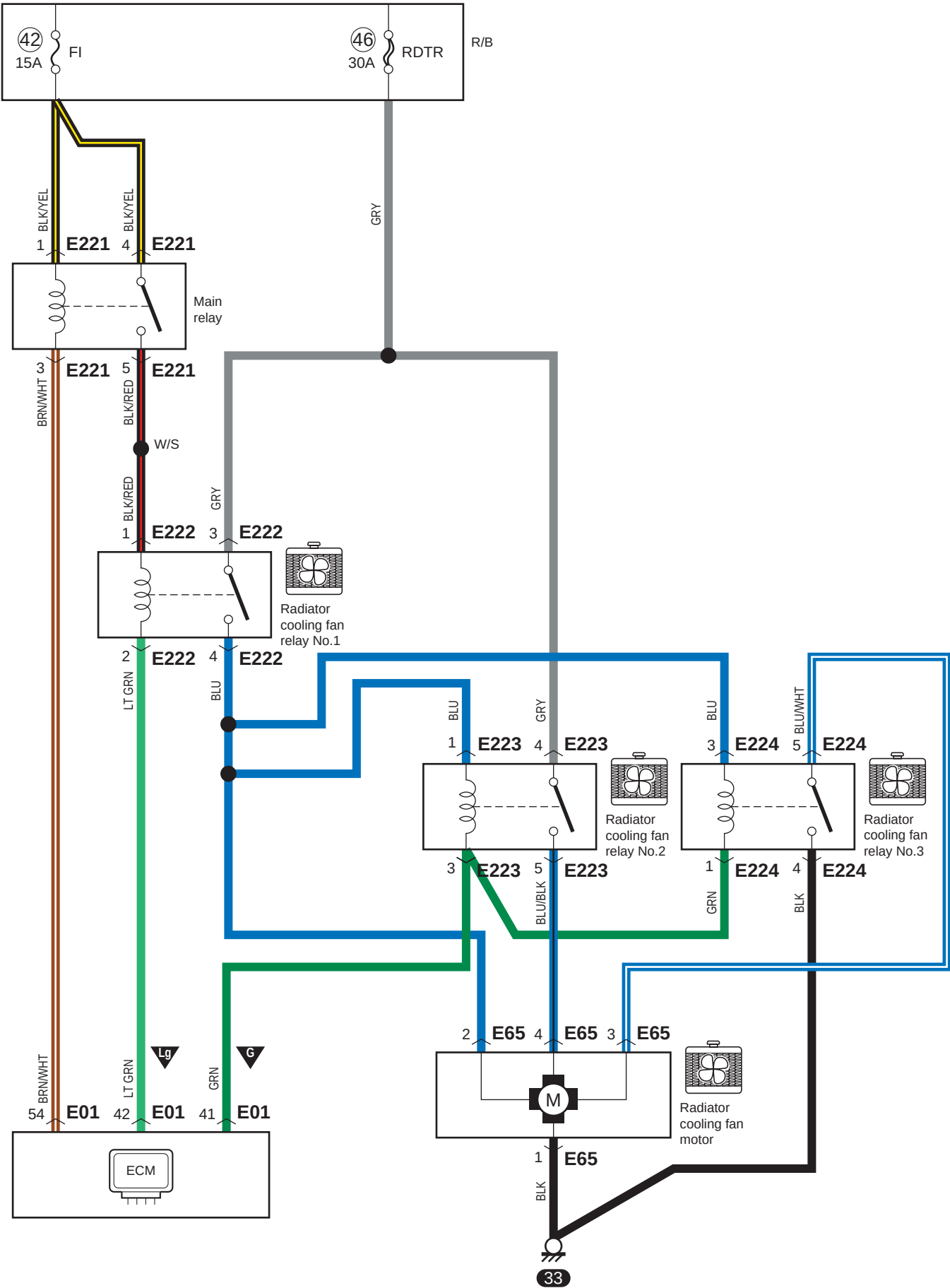
A-4-1 Cooling System Circuit Diagram (Petrol Model)
